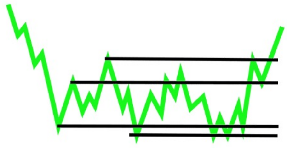
Wyckoff pattern
